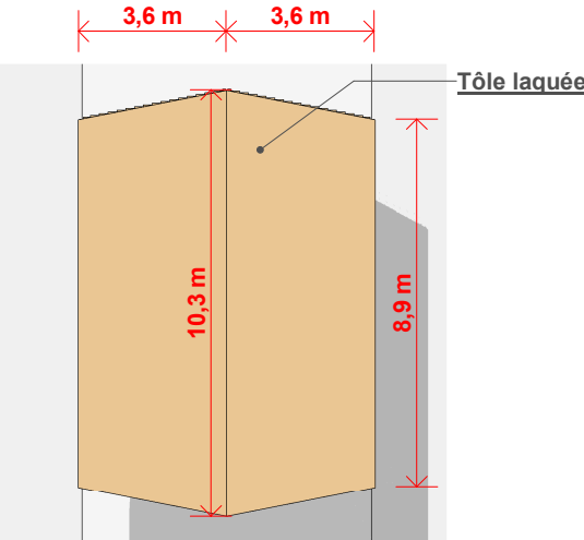
CARBET TYPE - PLAN
