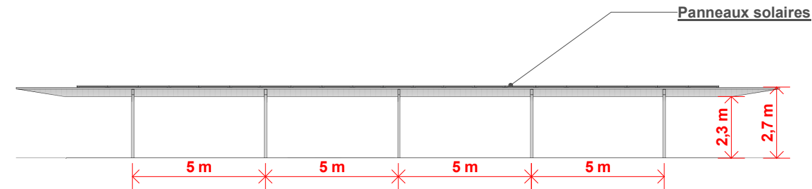
COUVERTURE PARKING TYPE - ELEVATION 1
