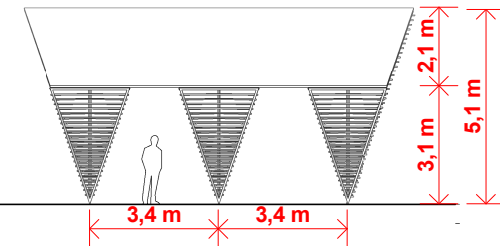
CARBET TYPE- ELEVATION 1
