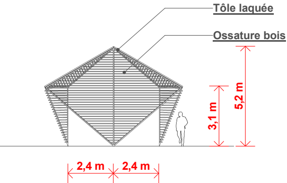
CARBET TYPE - ELEVATION 2
