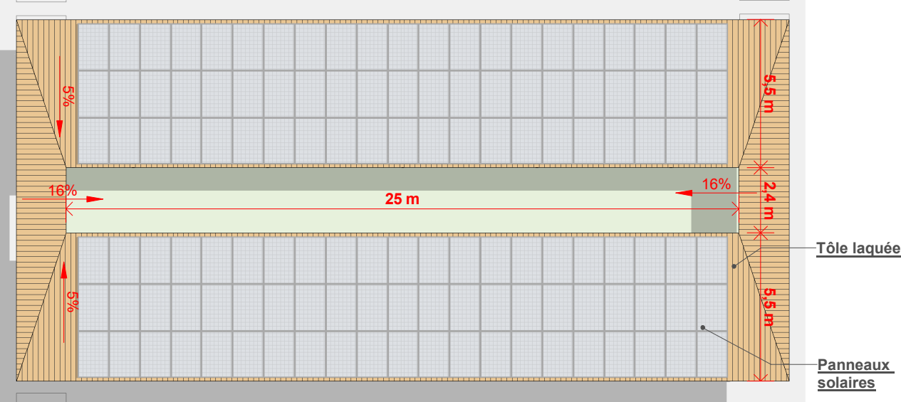
COUVERTURE TYPE PARKING - PLAN
