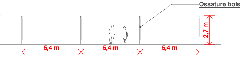
COUVERTURE CHEMINEMENT TYPE - ELEVATION 1
